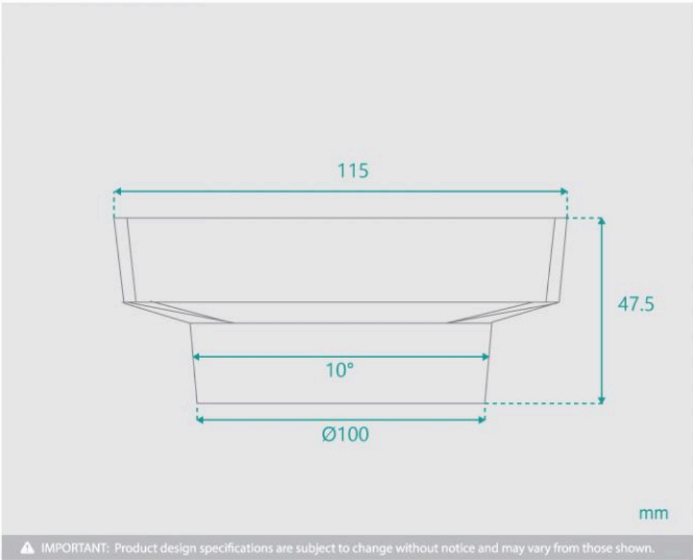
Shower / Floor Grate Tile Insert Waste (100mm) | G-0008
