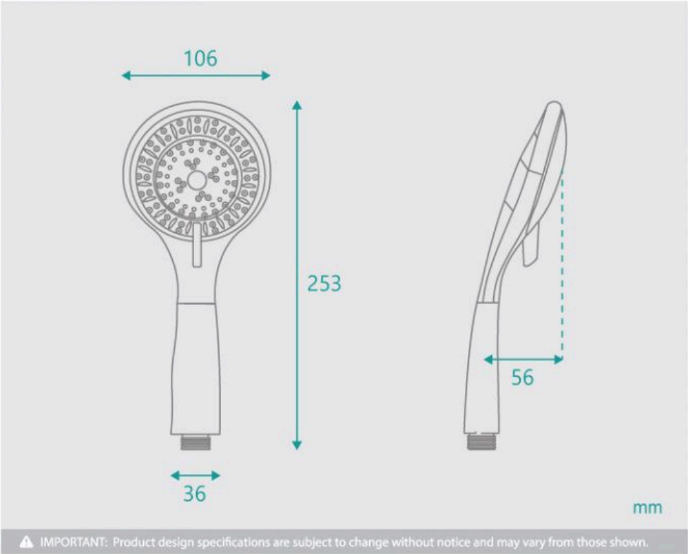
Eleanor Shower Hand Held 3 Function Black | S-1017
