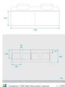
Frederick 1500 Wall Mounted Cabinet | J-2007
