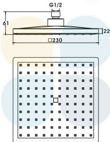
sebastian square shower head S-1001
