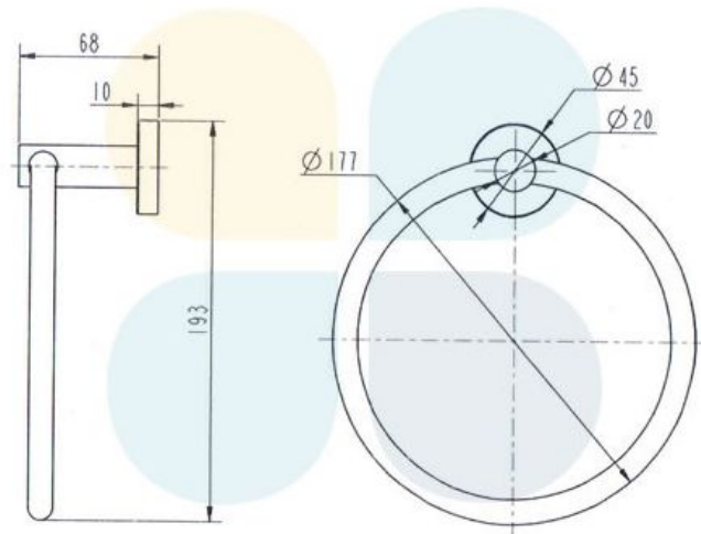
eleanor face towel holder A-1060
