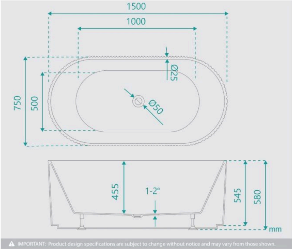
Harper 1500 Freestanding Bath Fluted Matte | B-4066
