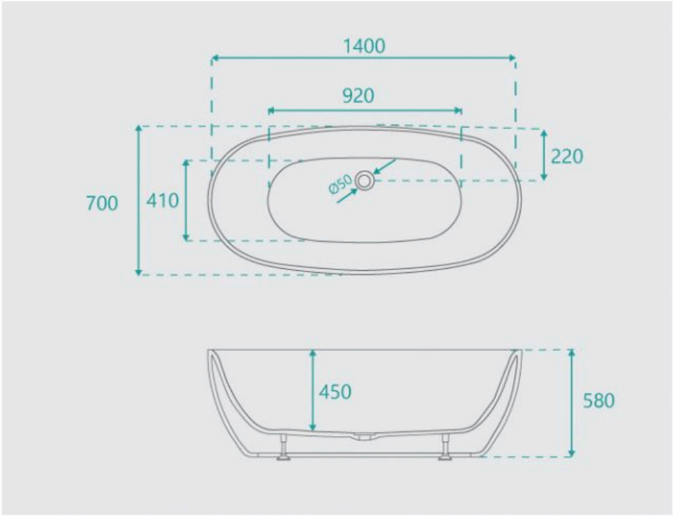
Ariana 1400 Freestanding Bath
