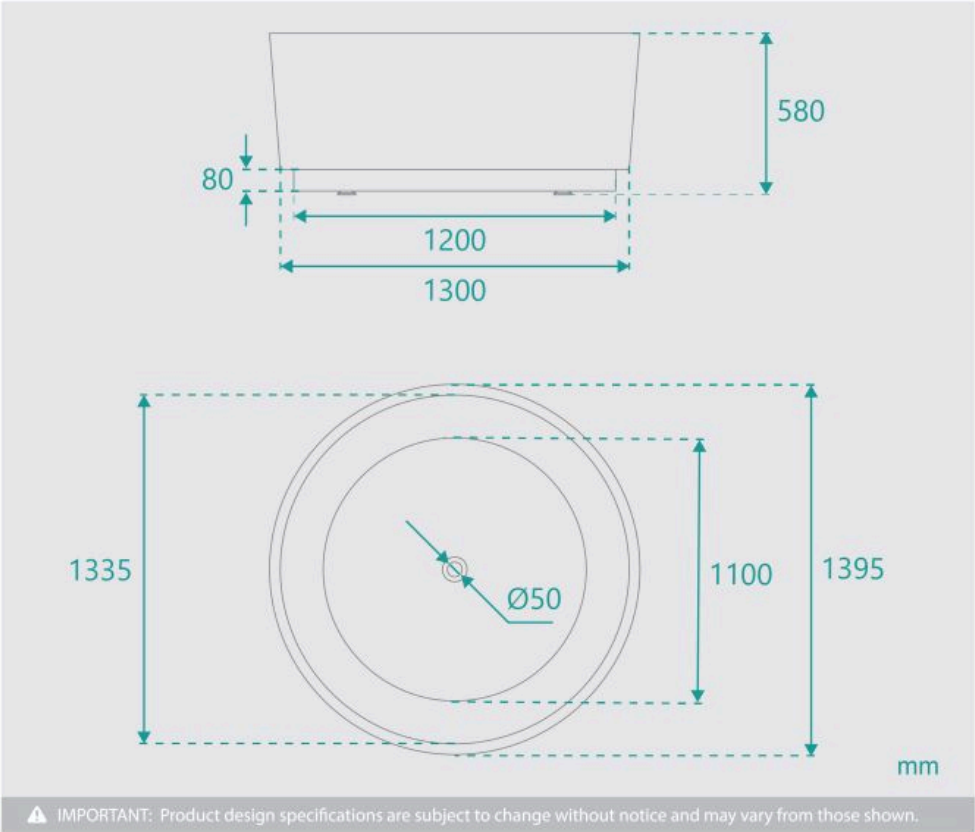
Harper Freestanding Round Bath 1400 Matte White | B-4068
