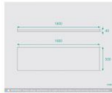
Vanity Benchtop 1800x500 Stone Upgrade
