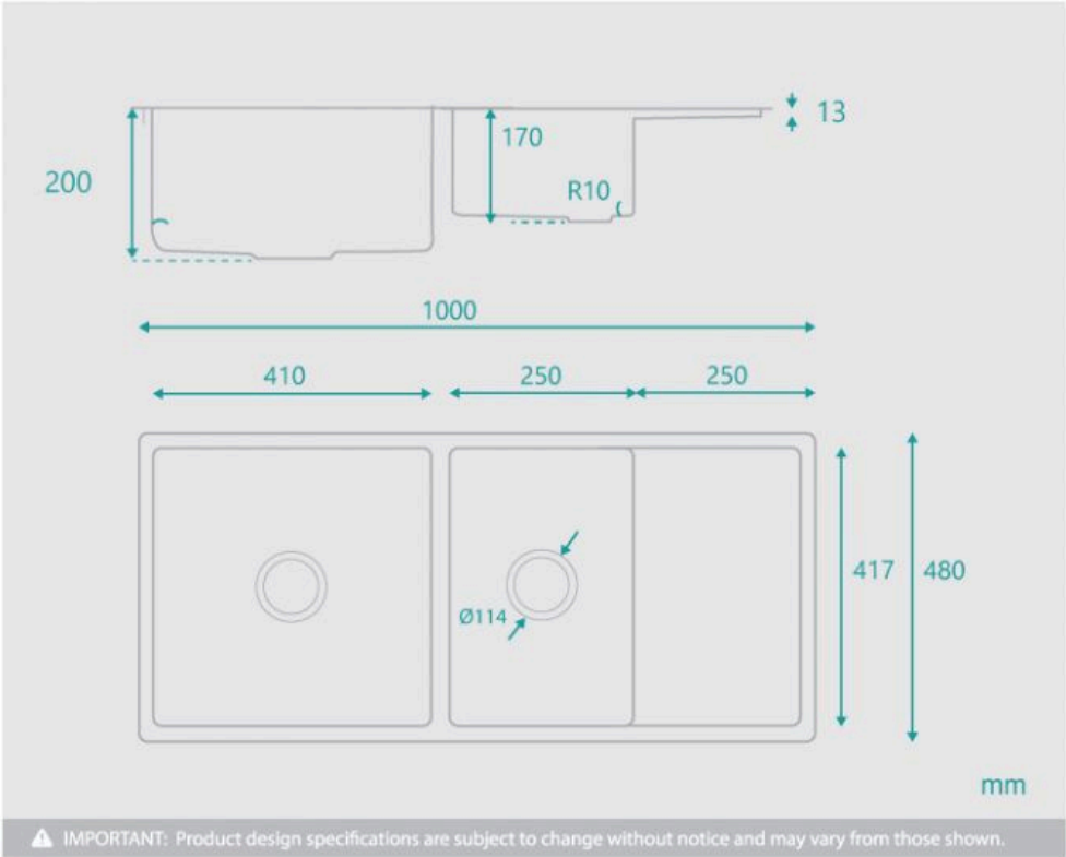
Toronto Double Square Kitchen Sink With Drainer | K-0209
