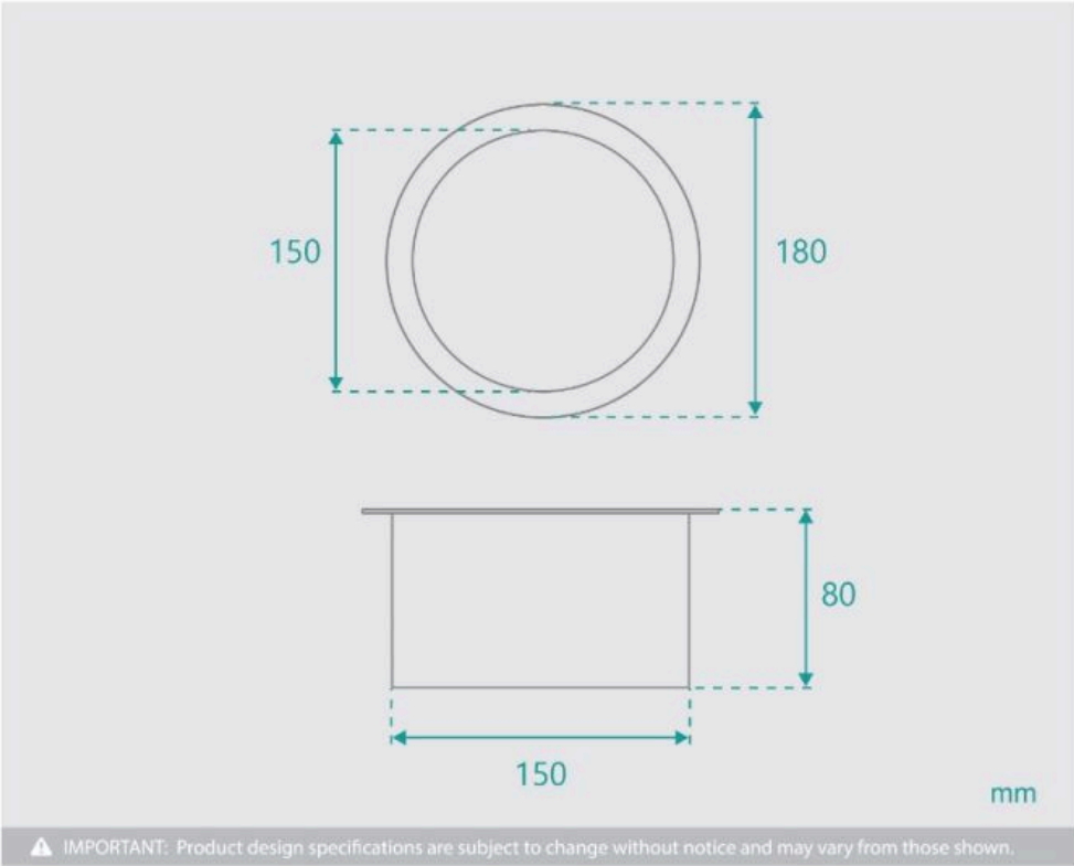
Round Stainless Steel Waste Chute with Lid | A-4101
